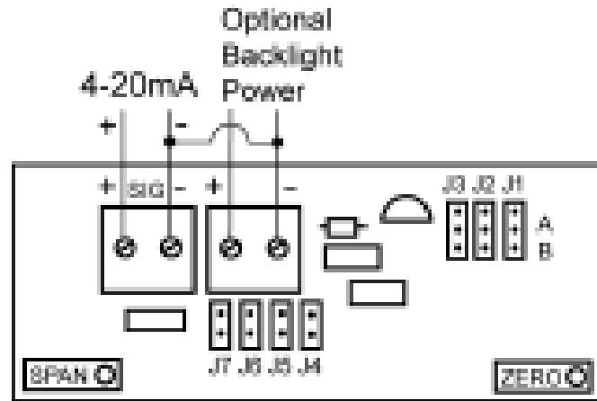
(upper) WIRING
