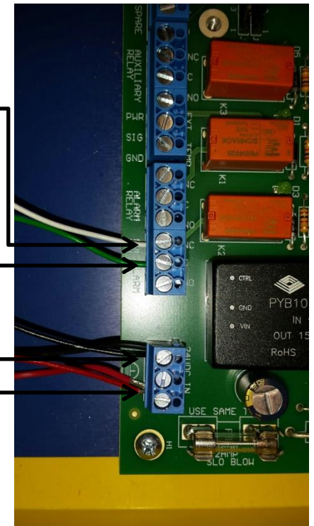
LBW-420-1 Relay connections
